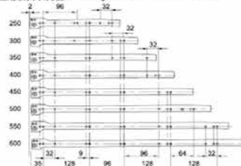
固定轨安装孔位 Fastening Position For Cabinet Member
