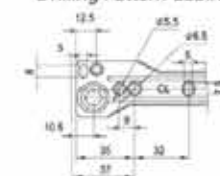
装配尺寸 Assembling Dimension
