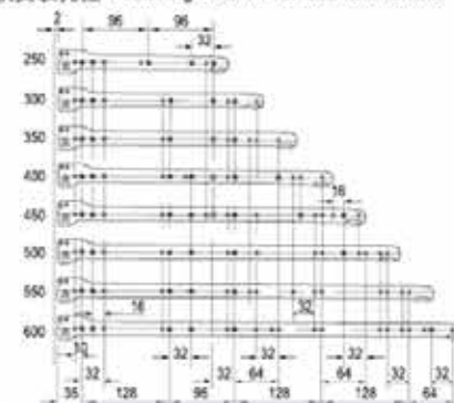
固定轨安装孔位 Fastening Position For Cabinet Member
