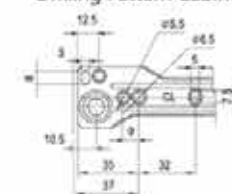
装配尺寸 Assembling Dimension
