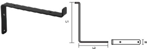
YLZC-39 HEAVY DUTY SHELF BRACKET
