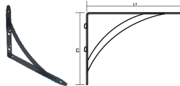
YLZC-53 SHELF BRACKET
