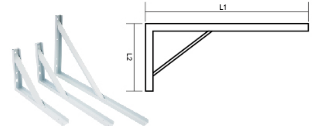
YLZC-49 HEAVY DUTY SHELF BRACKET
