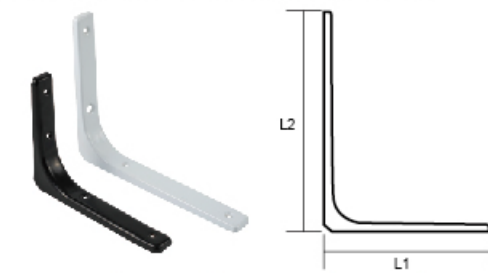
YLZC-32 HEAVY DUTY SHELF BRACKET
