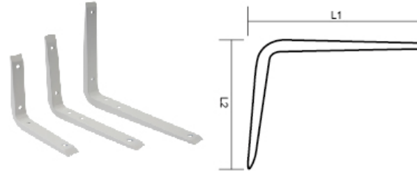
YLZC-61 HEAVY DUTY SHELF BRACKET
