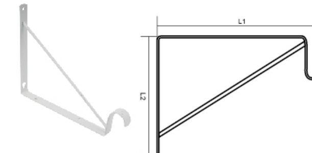
YLZC-60 HEAVY DUTY SHELF BRACKET
