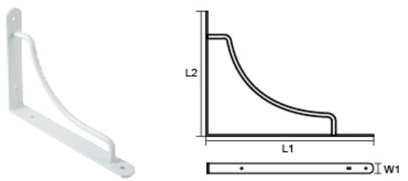
YLZC-36 DECORATIVE SHELF BRACKET
