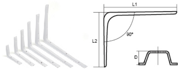
YLZC-23 A TYPE SHELF BRACKET
