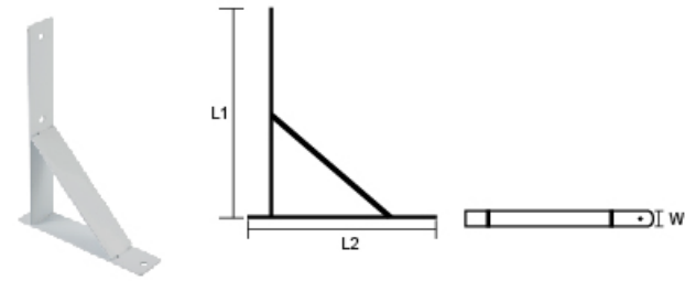
YLZC-33 HEAVY DUTY SHELF BRACKET
