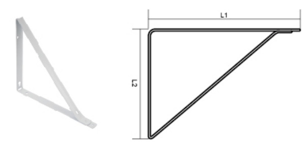
YLZC-59 HEAVY DUTY SHELF BRACKET
