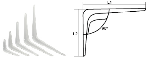
YLZC-31 A TYPE DEEP REINFORCE SHELF BRACKET
