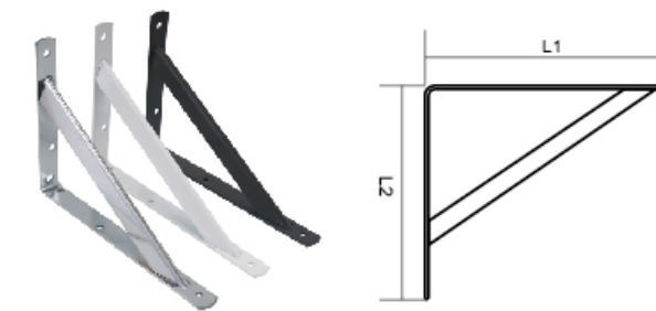
YLZC-48 HEAVY DUTY SHELF BRACKET
