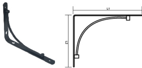
YLZC-52 SHELF BRACKET
