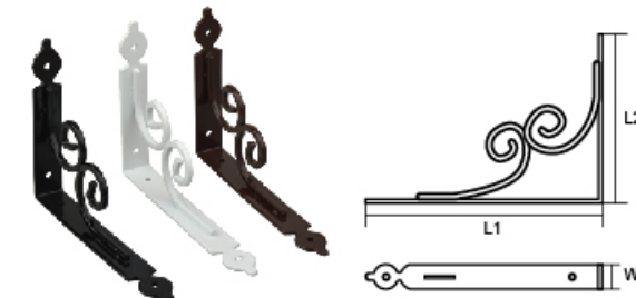
YLZC-20C S SHAPE DECORATIVE SHELF BRACKET
