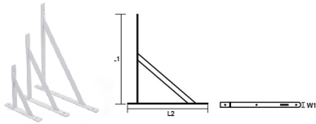
YLZC-27 HEAVY DUTY SHELF BRACKET
